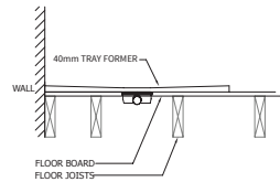
Trap recessed in the floor 40mm height
