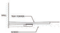
Trap and tray recessed in the floor Level access
