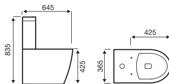
Close Coupled WC
